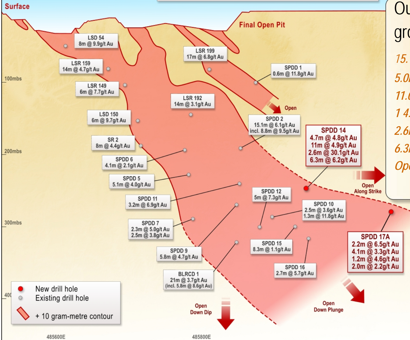
Sandpiper Deposit - Schematic Composite Long Section (showing significant down-hole intersections)
