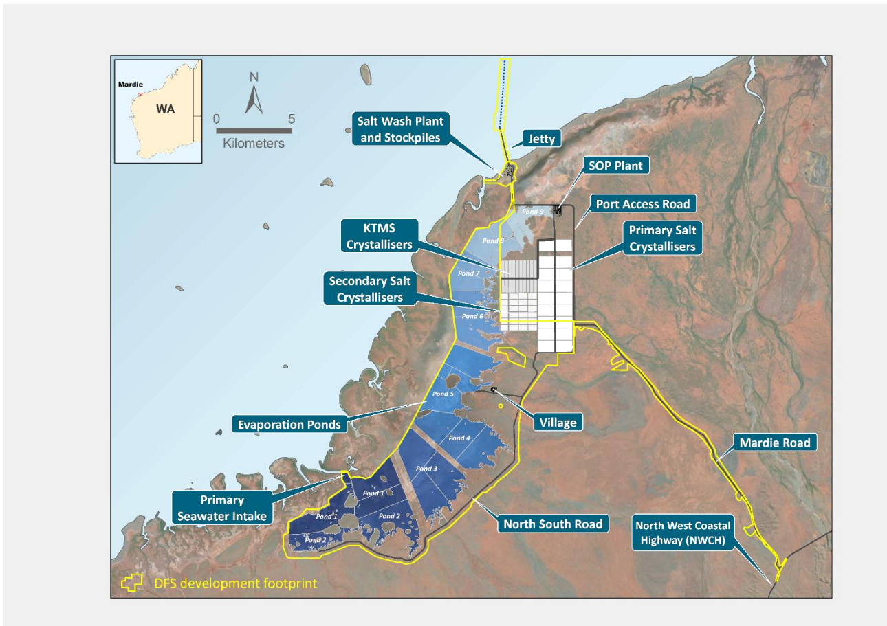
Figure 1: Project Layout and Development Envelope Covered by EPA Recommendation
