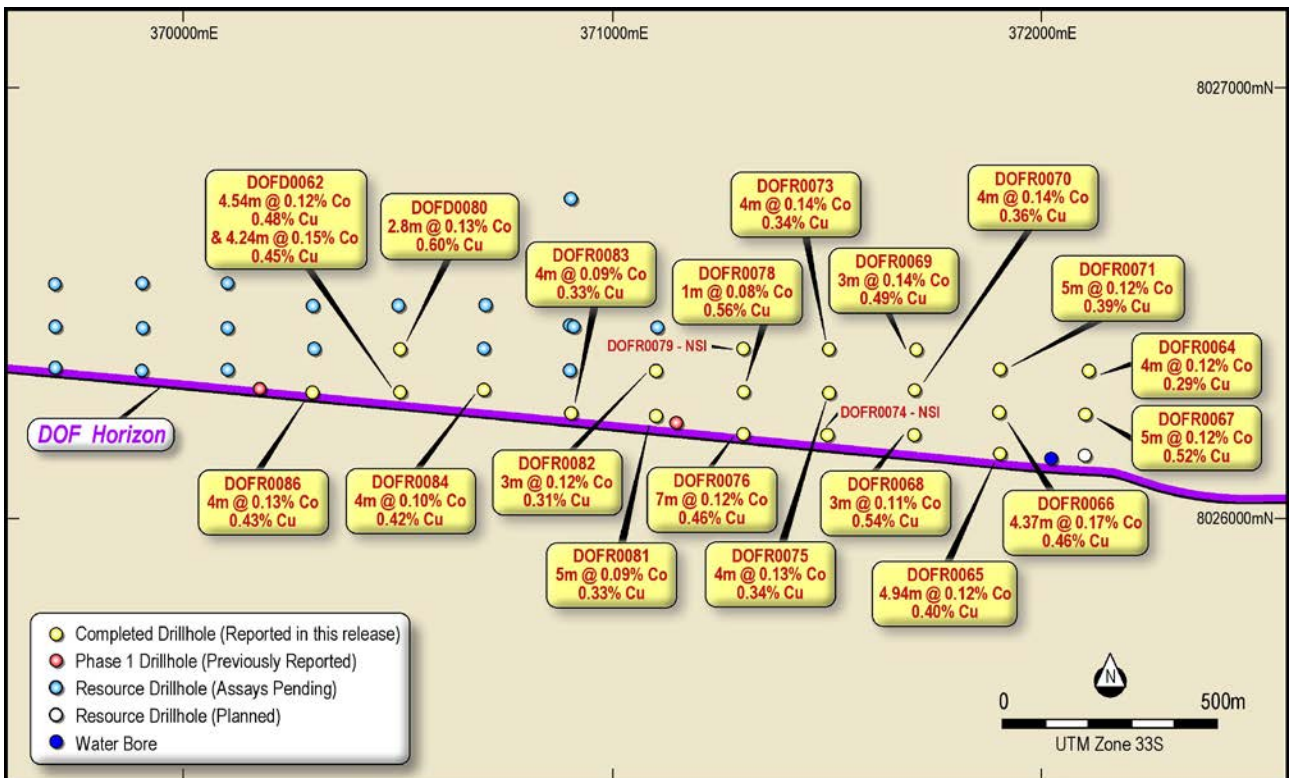
Figure 2: Resource Drilling Significant Intercepts
