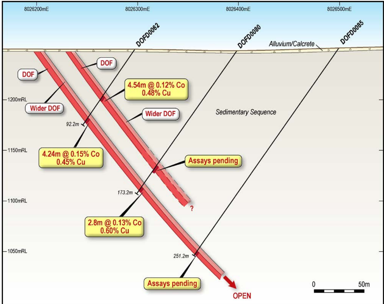
Figure 3: Cross Section 370,500 mE - Second Mineralised DOF Zone
