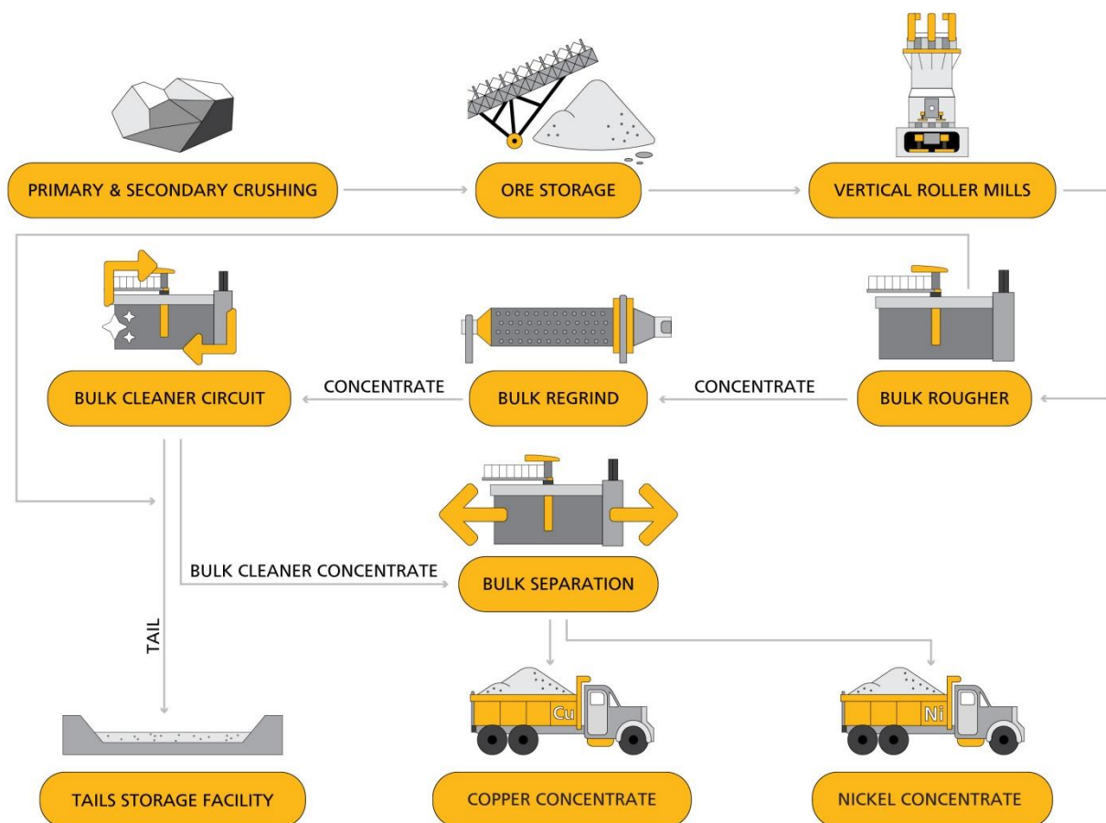
Figure 2: Flowsheet
