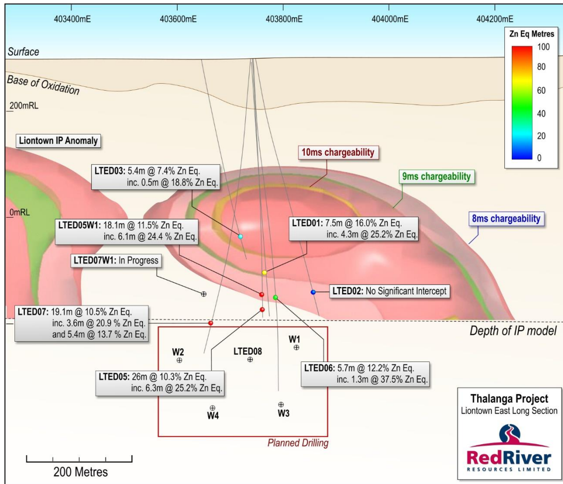
Figure 1 Liontown East Long Section
