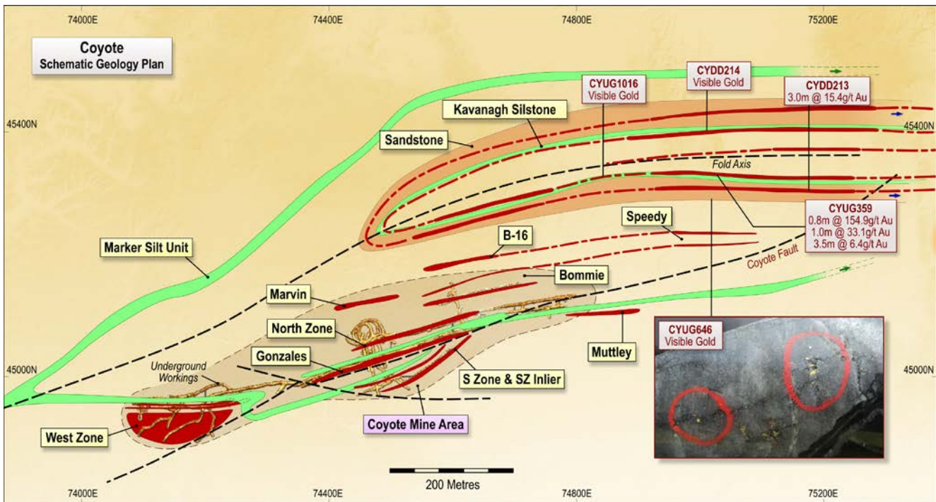
Figure 2: Coyote Schematic Geology Plan
