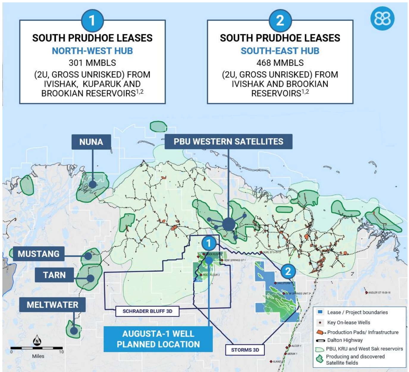
Figure 2: 88 Energy's North Slope position showing the planned location of the Augusta-1 exploration well.
