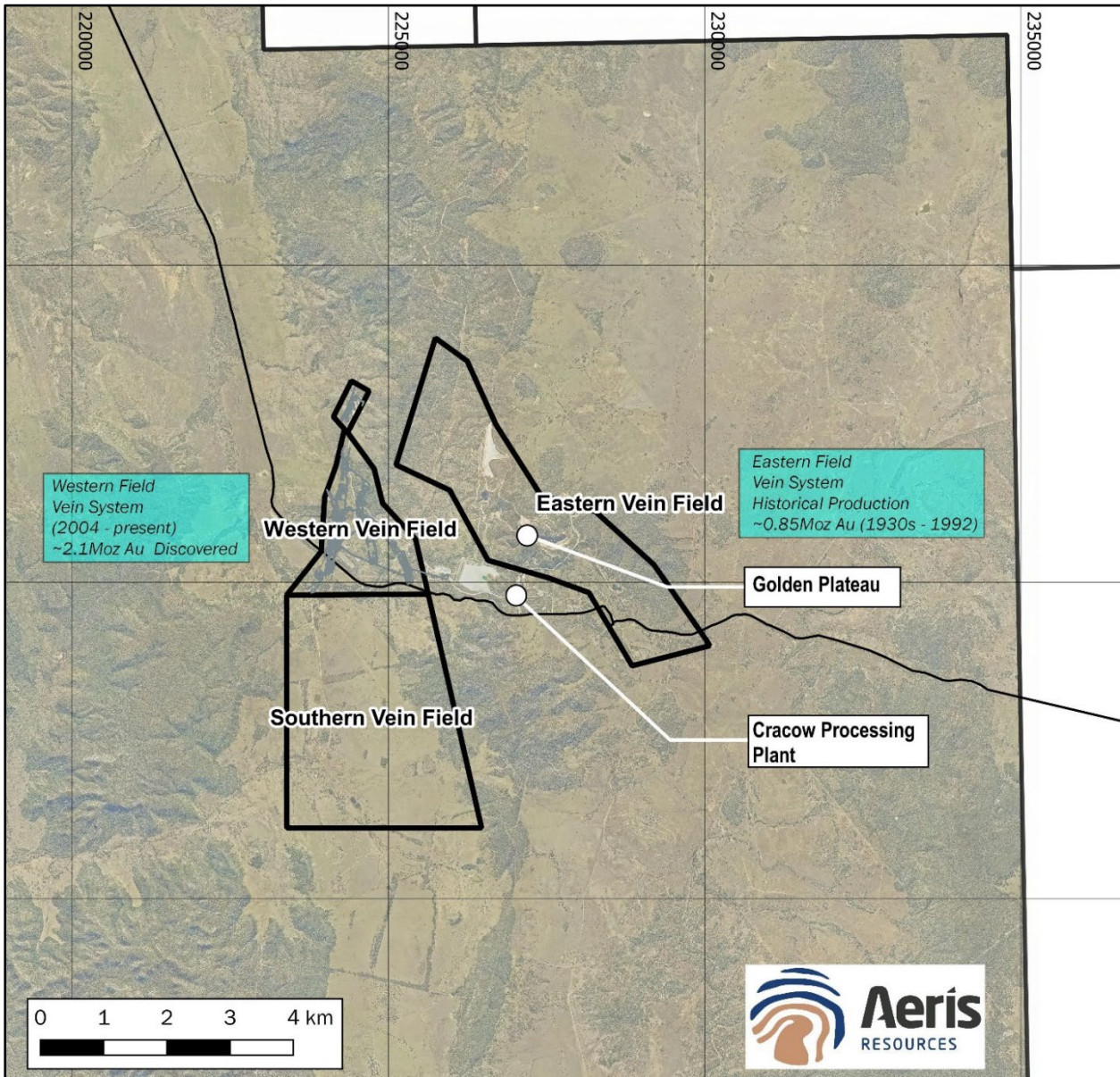
Figure 1 – Location map showing Golden Plateau deposit and Cracow processing plant.
