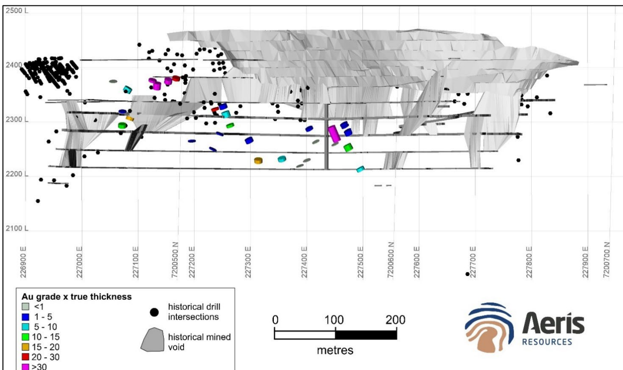
Figure 2 – Oblique view looking northeast showing drill hole intersections from the current drill program (coloured discs), historical workings (grey wireframes) and historical drill hole intersections (black dots).
