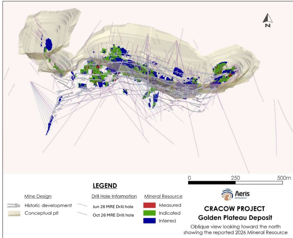
Figure 5: Oblique view of the October 2026 Golden Plateau MRE
