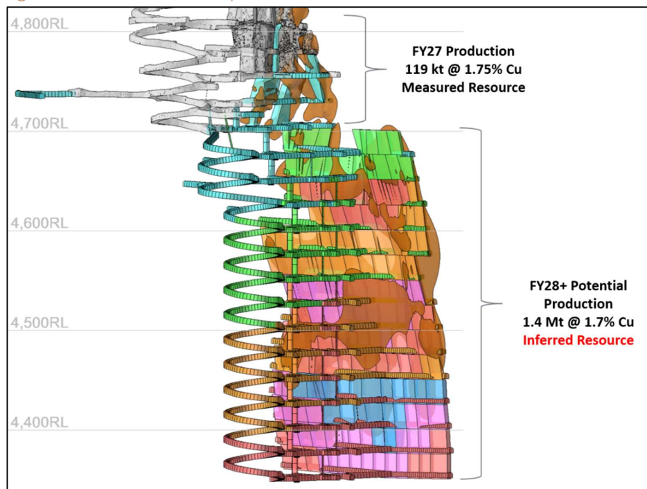
Figure 2: Avoca Tank mine plan
