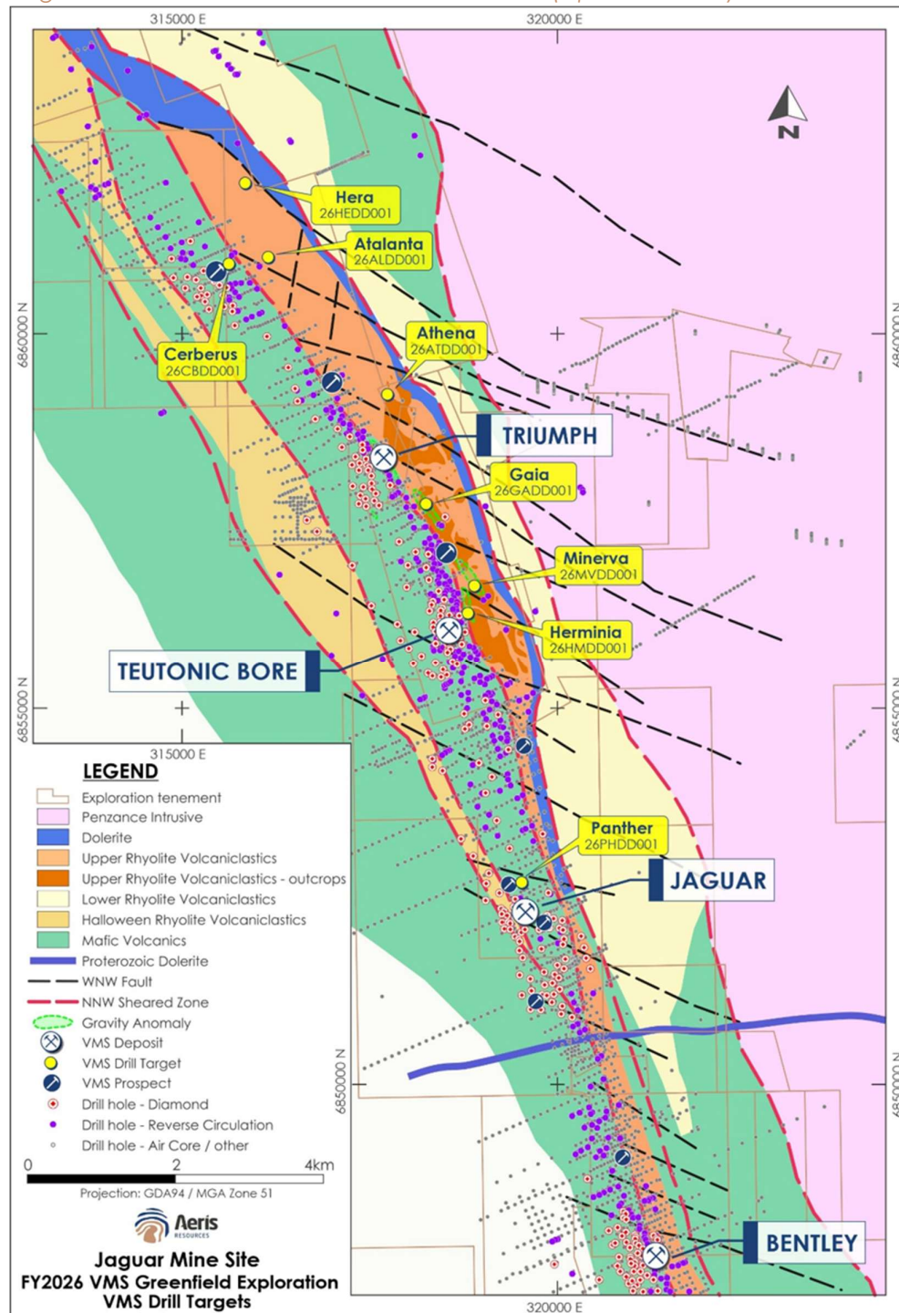
Figure 6: Regional geology across the known VMS corridor showing the location of the four known VMS deposits (Triumph, Teutonic Bore, Jaguar, and Bentley) and the eight priority drill targets that were diamond drill tested in Q4 FY26 (April-June 2026) 5
