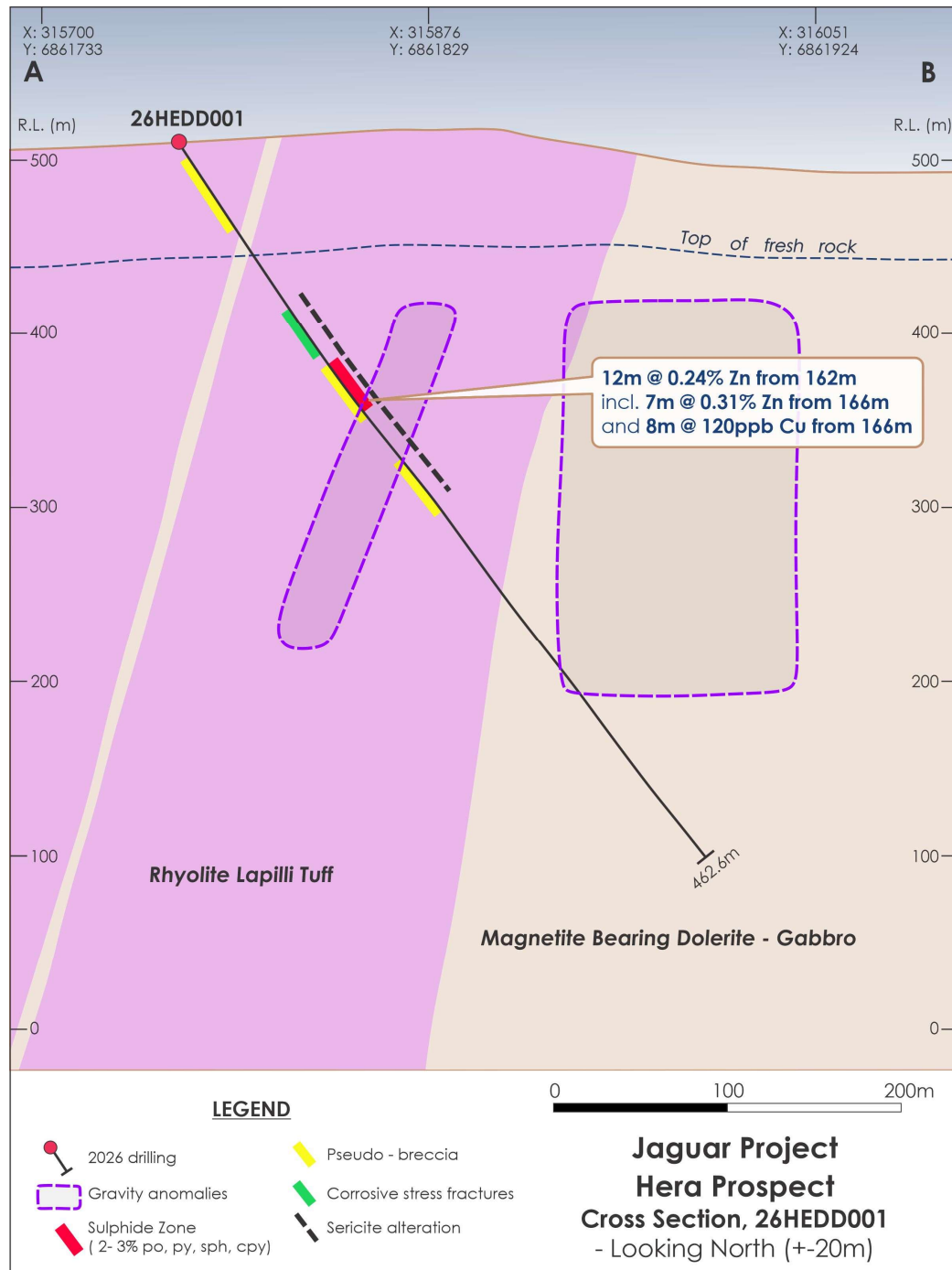
Figure 7: Interpreted geological section with drill hole results plotted for Hera prospect hole 26HEDD001
