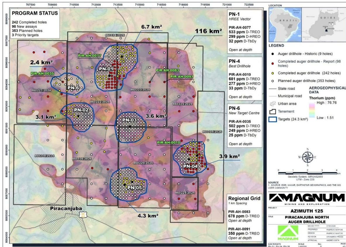
Figure 1 - Piracanjuba North multi-centre target framework showing PN-1, PN-4, PN-6 and regional 1,000 m grid context. The 116 km 2 figure is a geophysical target footprint and is not a drill-defined mineralised footprint, Exploration Target or Mineral Resource.
