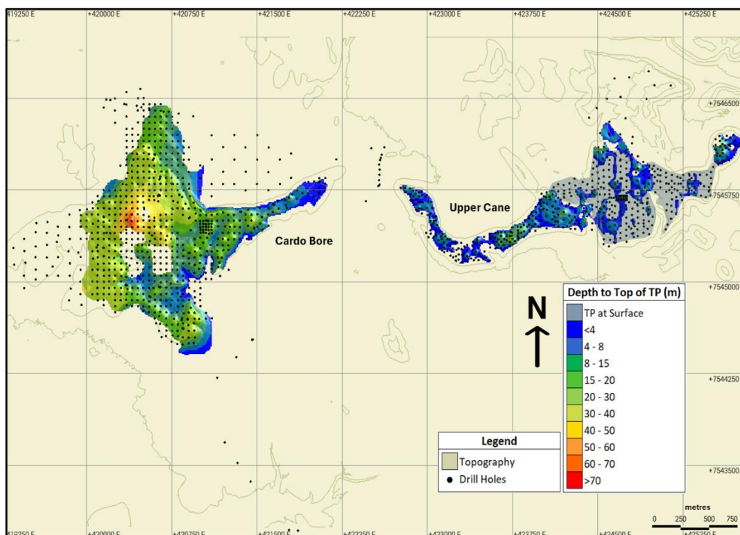
Figure 3: Cardo Bore and Upper Cane Plan View showing drill coverage and depth to the top of TP
