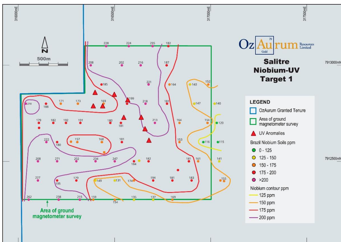
Figure 2: Target 1 niobium soil anomaly with proposed ground magnetometer survey
