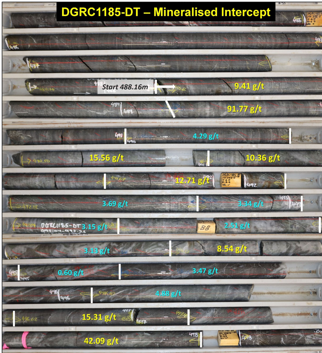
Figure 5a: Drill-core photos of DGRC1185-DT intercepting Never Never mineralisation from 488.16m downhole.
